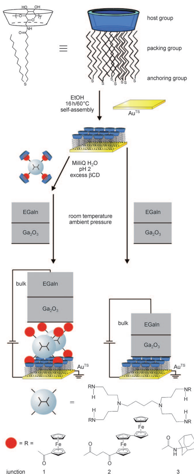
Figure 1. Fabrication process of the molecular junctions. The eutectic gallium–indium (EGaIn) is represented with a \text{Ga}_2\text{O}_3 layer on the surface.
